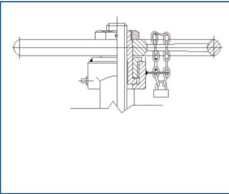
Locking device on the handwheel
