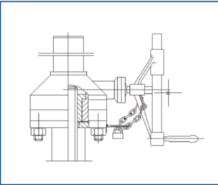
Locking device on the gear box
