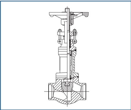
Forging steel bellows sealed valves
