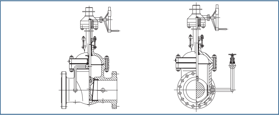
Special by-pass application
