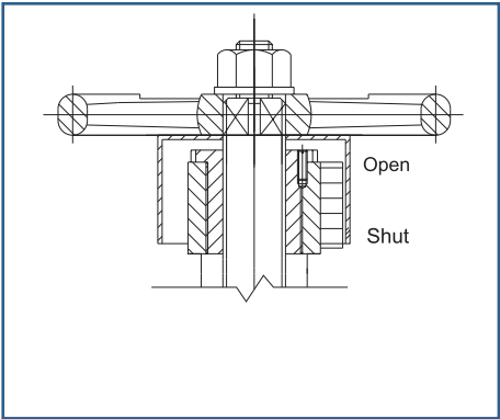
Position indicator on globe valves
