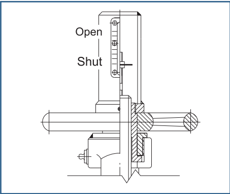
Position indicator on gate valves
