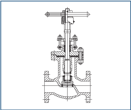
Casting steel bellows sealed valves
