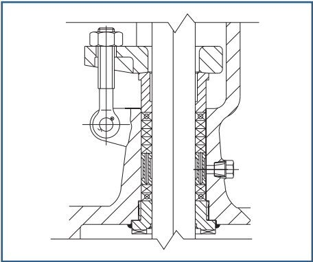
The lantern on the gate and globe valves
